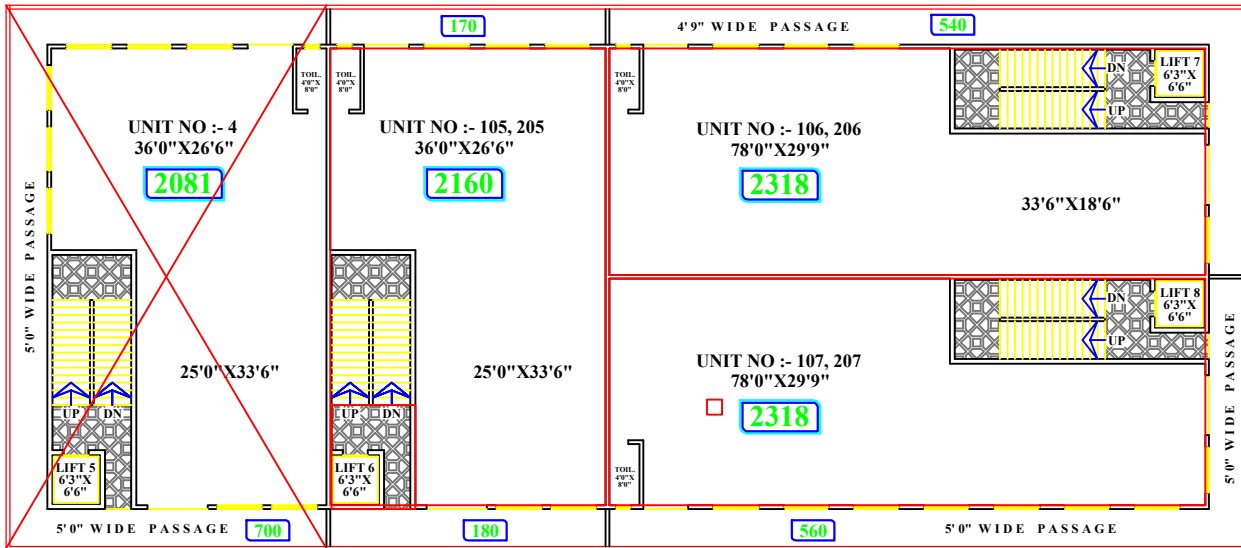
1ST & 2ND FLOOR PLAN
